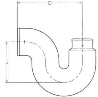
REDUCING P-TRAP
