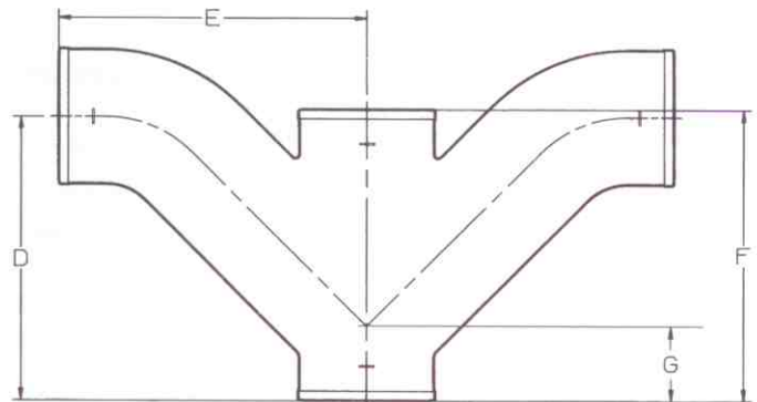
DOUBLE COMBINATION
