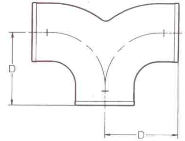
DOUBLE QUARTER BEND
