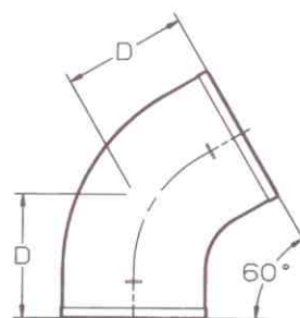
SIXTH BEND
