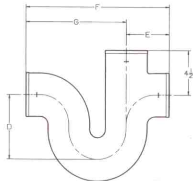
RUNNING TRAP w/4" SINGLE VENT
