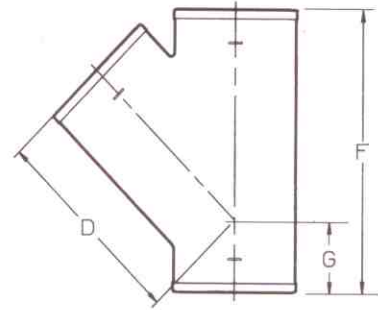
WYE
