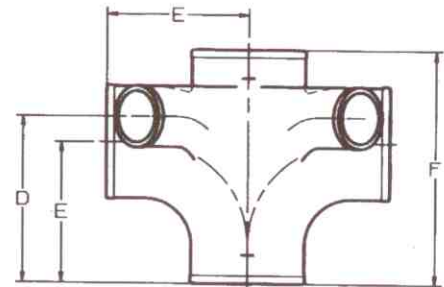
SAN CROSS (with two 2" 45° San Openings—Same Side) New Orleans Code (No Baffle)
