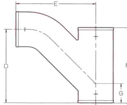
COMBINATION
